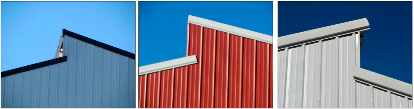
Figure 37. An overshoot roof can provide reasonable air removal when the opening is high enough as depicted in these barns. However, good air removal only occurs when wind moves across the higher side. When wind moves toward the opening, the wind actually forces air back into the barn. This design is not generally recommended.
