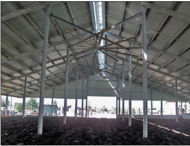
Figure 42. High volume, low speed fans have been added to many compost bedded pack barns. These fans distribute air well across a wide area.
