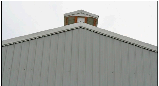
Figure 33. A ridge vent with a cap provides nearly as much air removal as the upstand with less chance of precipitation entering the barn. This design removes more air from the barn regardless of wind direction. Though this ridge vent may cost more than the overshoot design, the benefits to the pack and cow performance easily outweigh the cost over the barn's lifetime.
