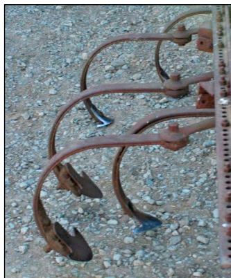
Figure 53. Sweeps or shovels may be added to tillage implement tines to provide more effective stirring. This is a cheap, effective addition to existing implements.
