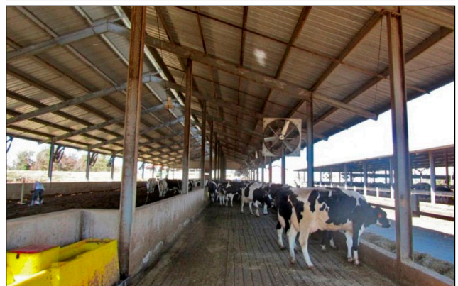
Figure 16. Wide alleys improve cow flow, minimize the risk of cow injury, and allow easy access to feed and water.
