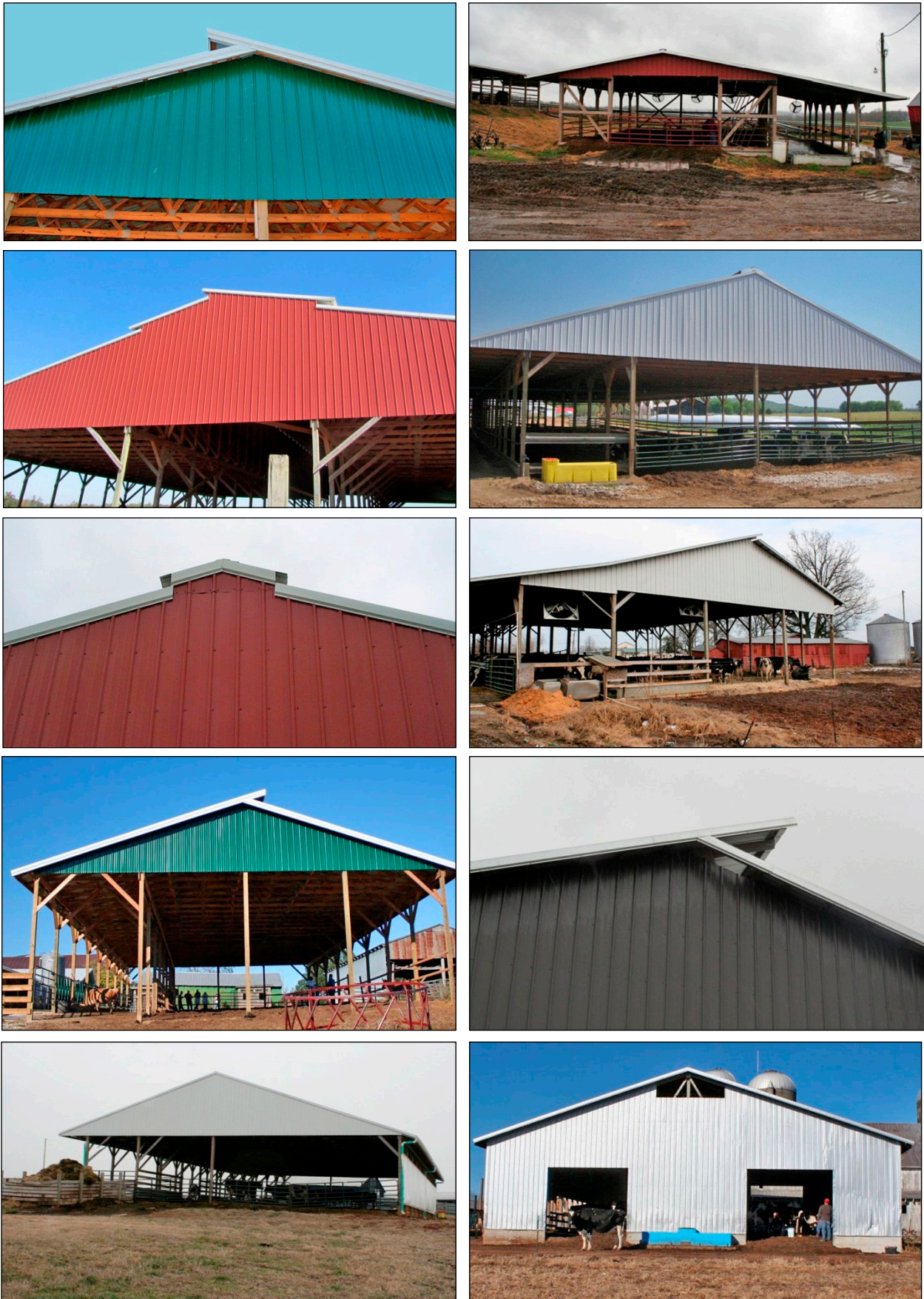
Figure 40. Each of these barns suffers from the same design flaw. In each case, the ridge opening restricts air removal from the top of the barn.
