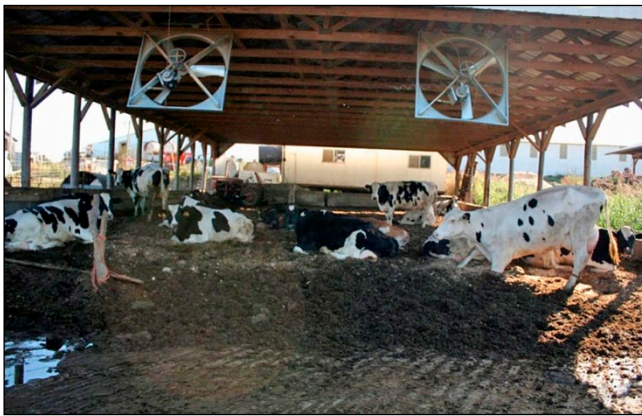
Figure 18. To minimize wetness, build multiple, narrow entrances along the long side of the barn. Entrances should be spaced every 50 feet.
