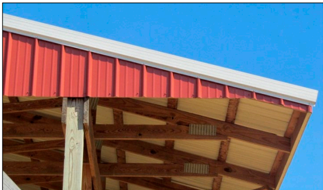
Figure 29. Short eave overhangs increase the likelihood of precipitation entering the pack and creating wet areas.
