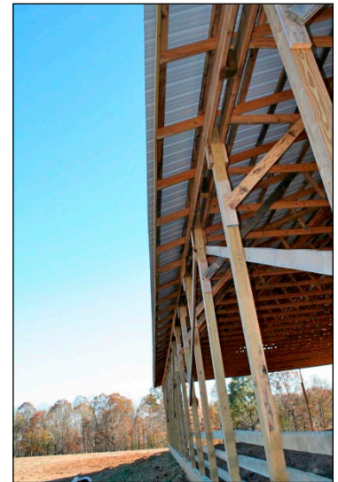
Figure 29. Short eave overhangs increase the likelihood of precipitation entering the pack and creating wet areas.
