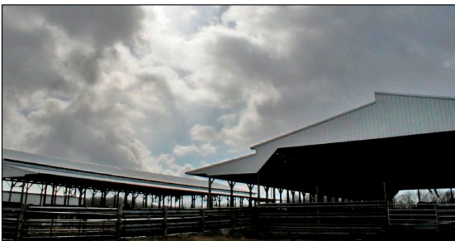
Figure 6 . These barns were constructed too close together. Neighboring barns should have at least 100 feet between them to maximize airflow.
