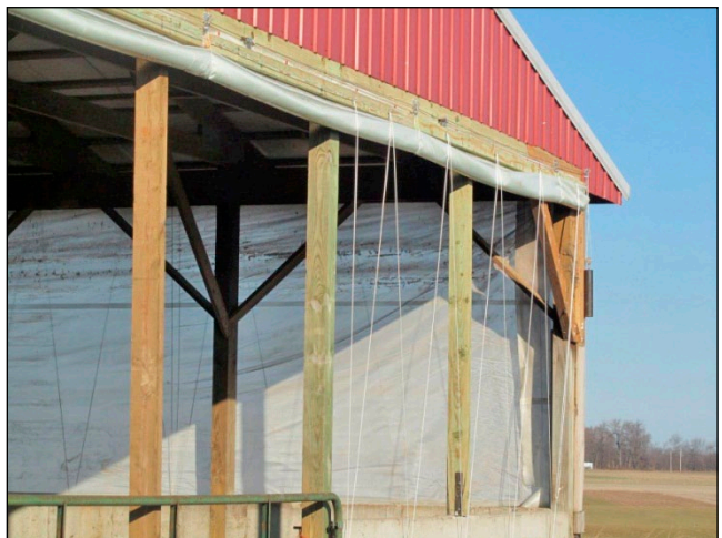
Figure 30. Cold winds blowing across the pack quickly remove the heat needed for composting. Thus, curtains are recommended in the winter. Curtains should be placed at least on the side with predominant winds.
