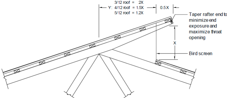
Figure 38. Design of an overshoot ridge. 3 inches of opening (x) for every 10 feet of building width (minimum 12 inches). This design is not preferred.
